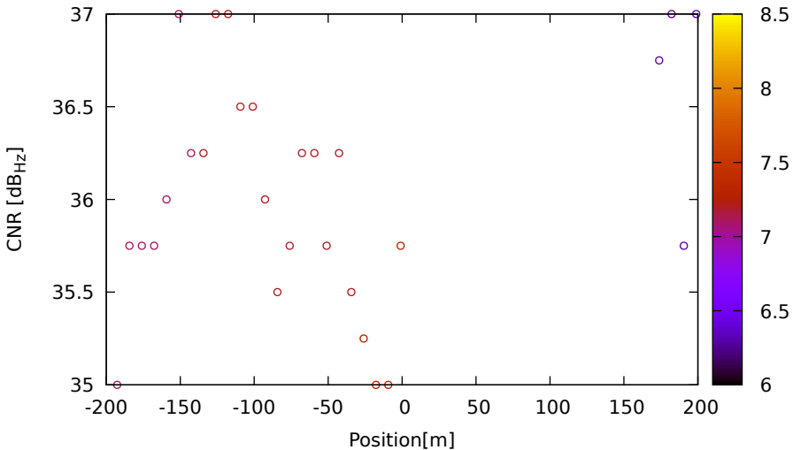
CNR vs position for R17 (G2) on LeicaGS18 - DOY 262 jam. 3
