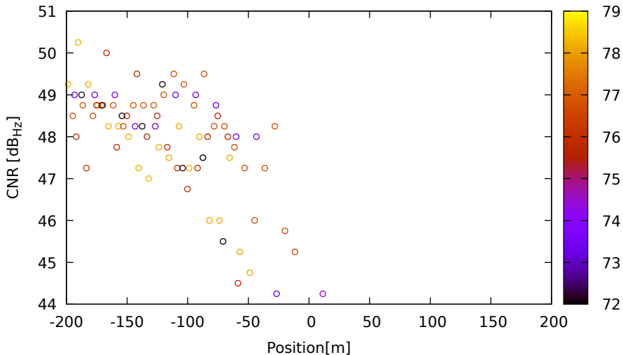
CNR vs position for R23 (G1) on LeicaGS18 - DOY 262 jam. 2
