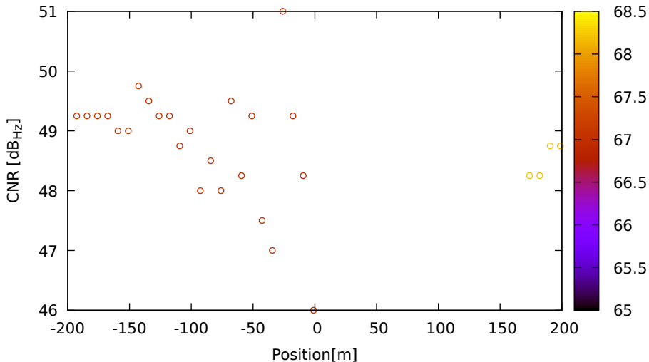
CNR vs position for R23 (G1) on LeicaGS18 - DOY 262 jam. 3
