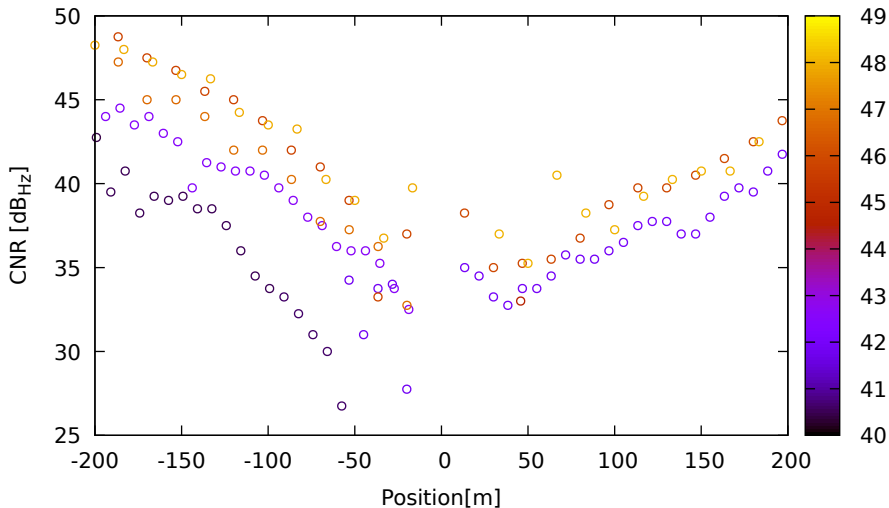
CNR vs position for R24 (G1) on LeicaGS18 - DOY 262 jam. 1
