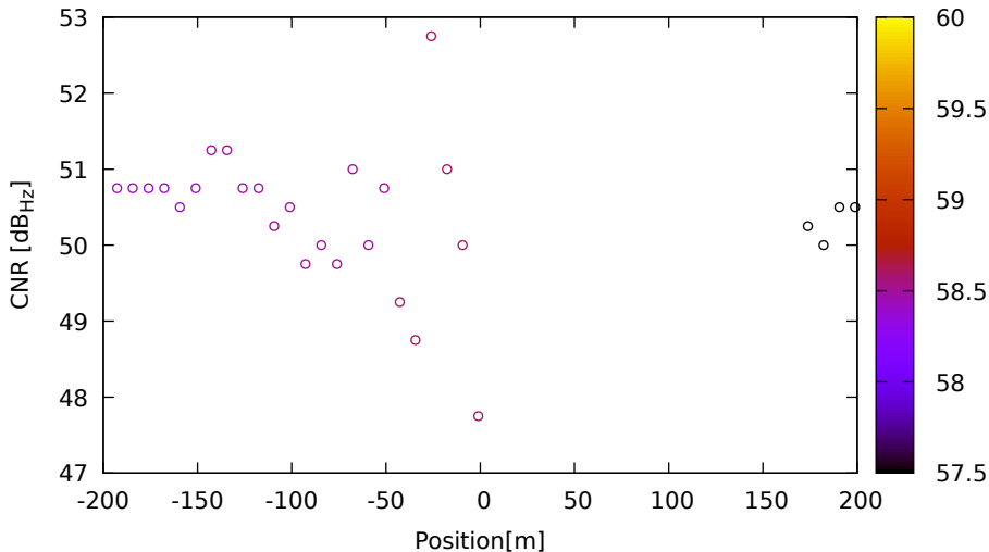
CNR vs position for R24 (G1) on LeicaGS18 - DOY 262 jam. 3
