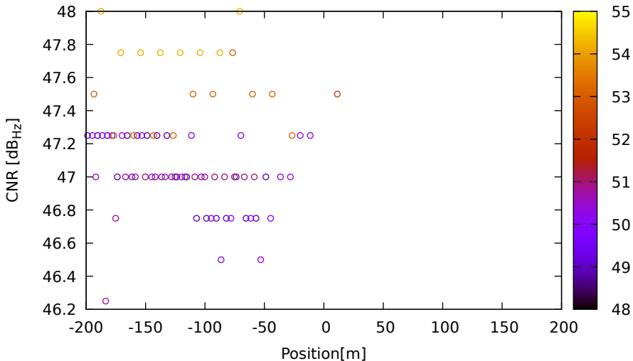
CNR vs position for R24 (G2) on LeicaGS18 - DOY 262 jam. 2
