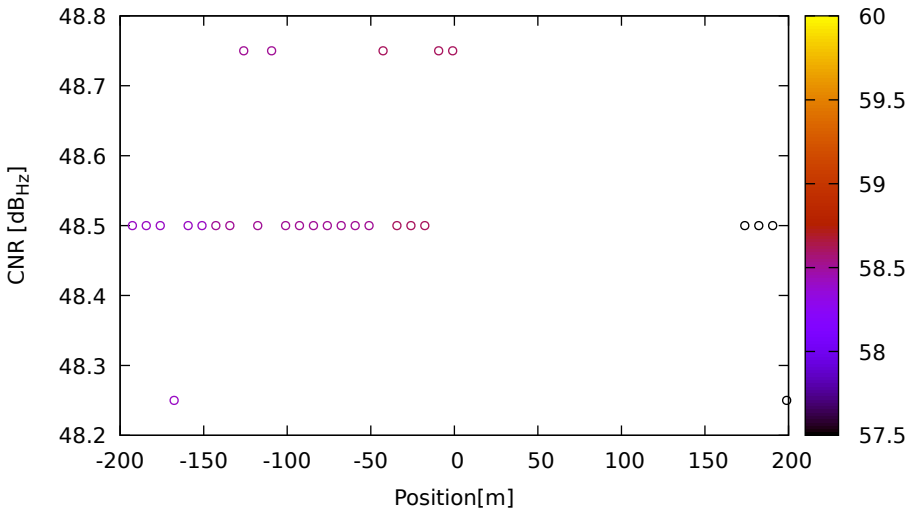
CNR vs position for R24 (G2) on LeicaGS18 - DOY 262 jam. 3
