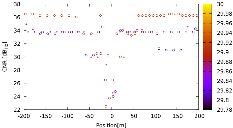
CNR vs position for C06 (B1) on Xiaomi11T - DOY 262 jam. 1
