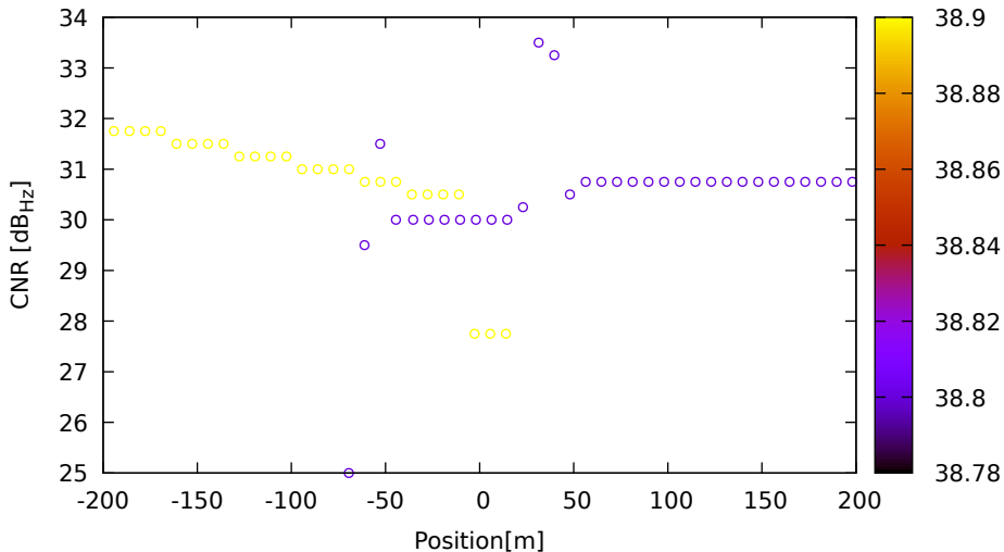
CNR vs position for C09 (B1) on Xiaomi11T - DOY 262 jam. 3
