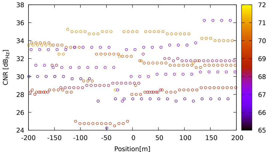
CNR vs position for C14 (B1) on Xiaomi11T - DOY 262 jam. 2
