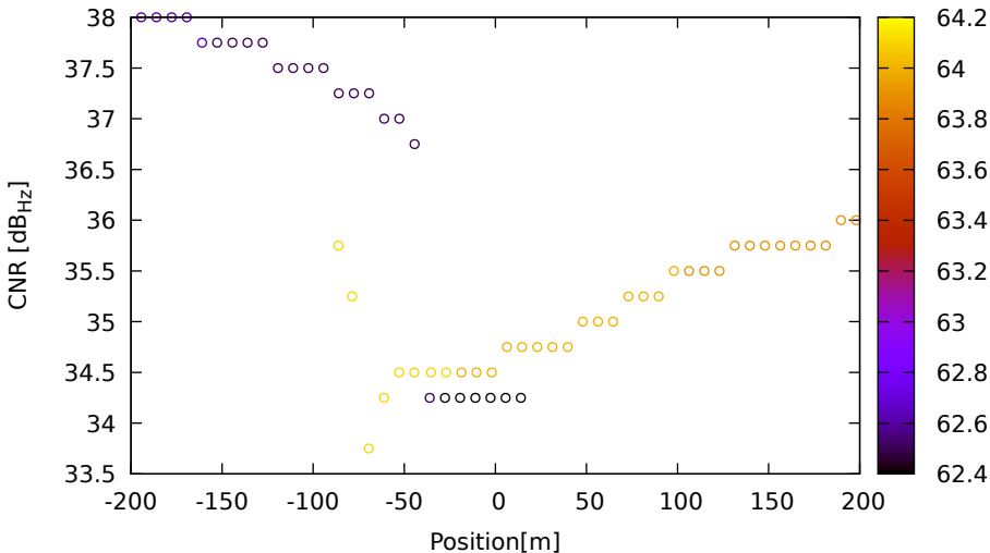
CNR vs position for C14 (B1) on Xiaomi11T - DOY 262 jam. 3
