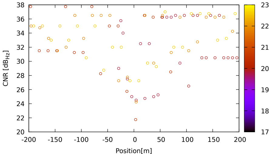
CNR vs position for C27 (B1) on Xiaomi11T - DOY 262 jam. 1
