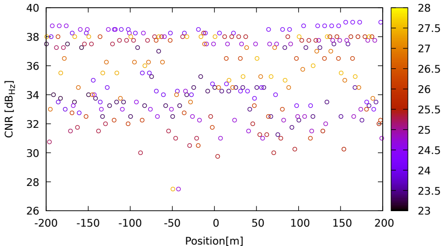
CNR vs position for C27 (B1) on Xiaomi11T - DOY 262 jam. 2
