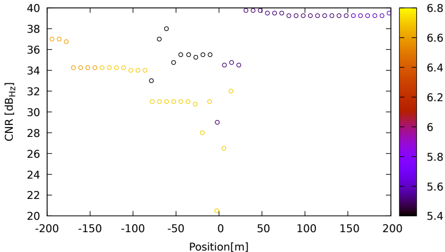
CNR vs position for E03 (E1) on Xiaomi11T - DOY 262 jam. 3
