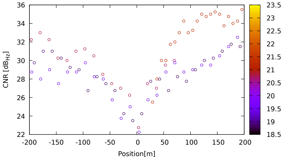
CNR vs position for E04 (E5a) on Xiaomi11T - DOY 262 jam. 1
