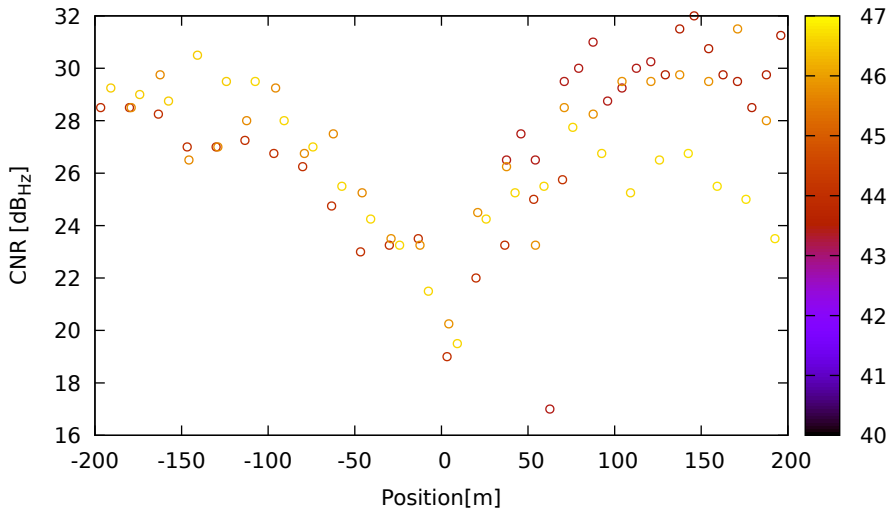
CNR vs position for E05 (E5a) on Xiaomi11T - DOY 262 jam. 1
