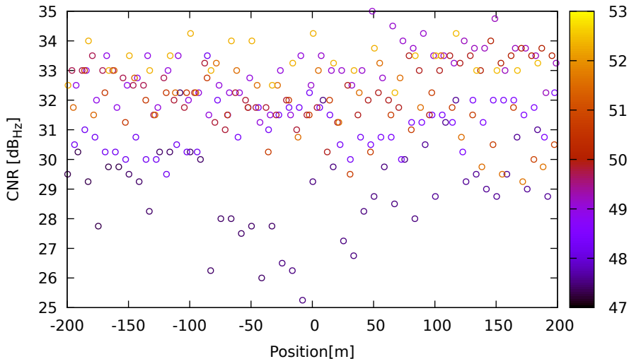
CNR vs position for E05 (E5a) on Xiaomi11T - DOY 262 jam. 2
