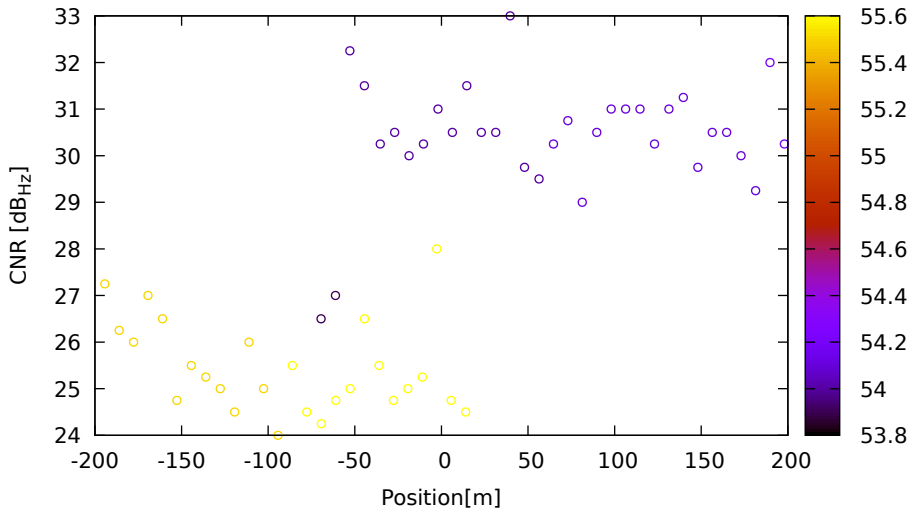
CNR vs position for E05 (E5a) on Xiaomi11T - DOY 262 jam. 3
