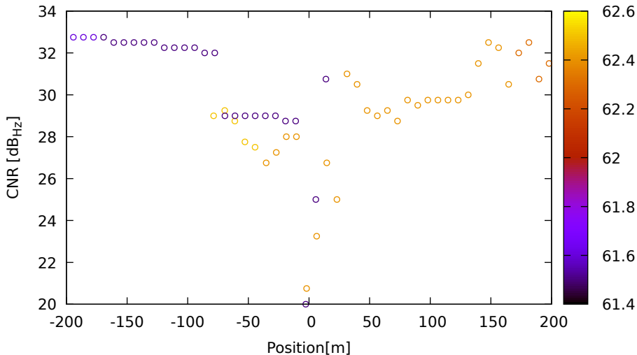
CNR vs position for E09 (E1) on Xiaomi11T - DOY 262 jam. 3
