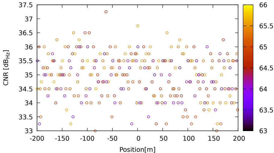
CNR vs position for E09 (E5a) on Xiaomi11T - DOY 262 jam. 2
