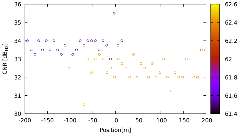
CNR vs position for E09 (E5a) on Xiaomi11T - DOY 262 jam. 3
