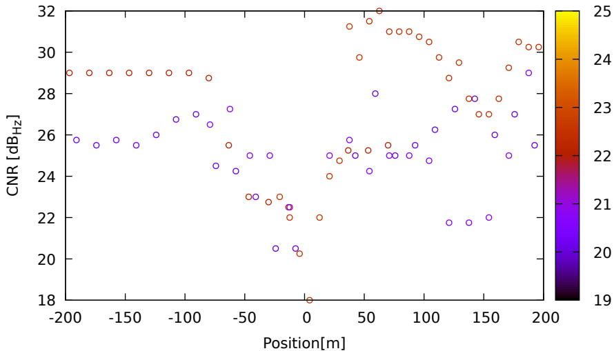
CNR vs position for E11 (E1) on Xiaomi11T - DOY 262 jam. 1
