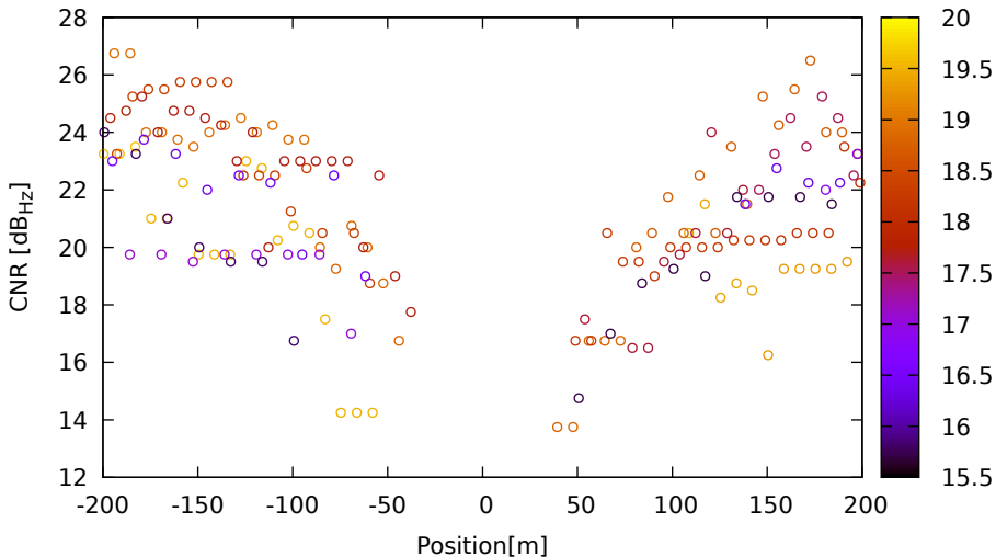
CNR vs position for E11 (E1) on Xiaomi11T - DOY 262 jam. 2
