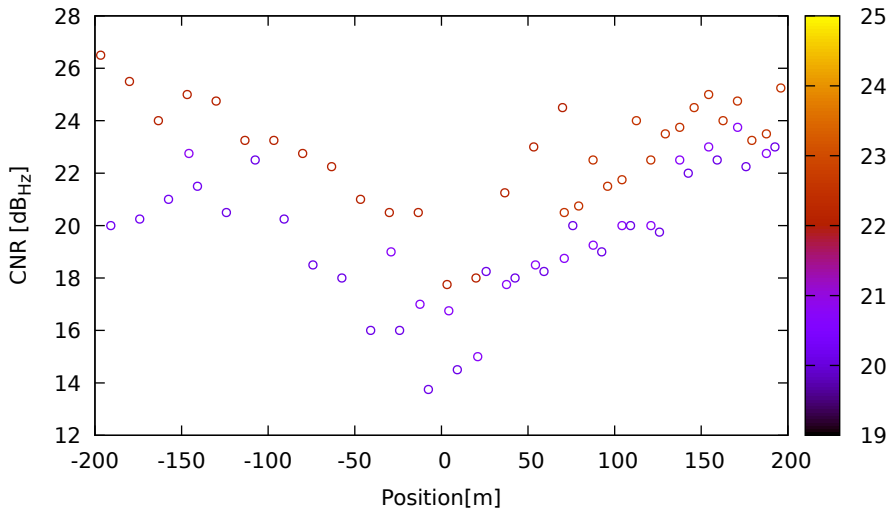
CNR vs position for E11 (E5a) on Xiaomi11T - DOY 262 jam. 1
