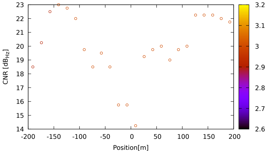
CNR vs position for E15 (E5a) on Xiaomi11T - DOY 262 jam. 1
