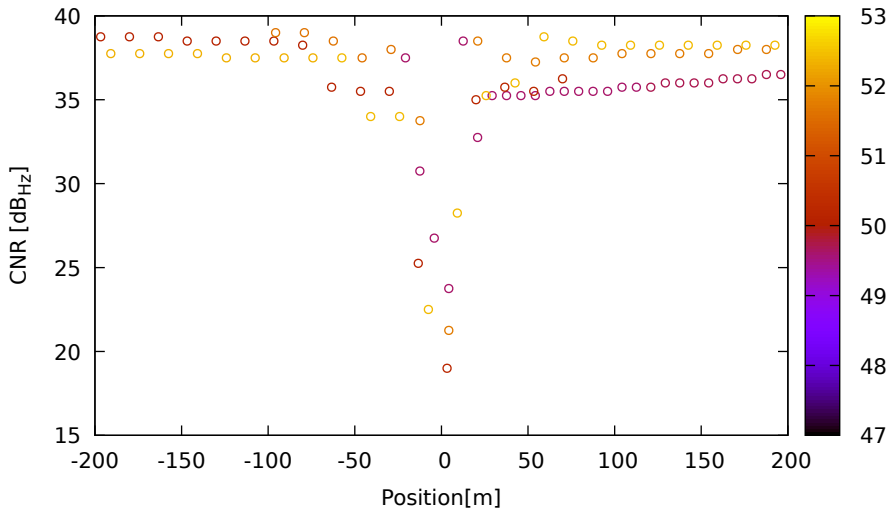
CNR vs position for E34 (E1) on Xiaomi11T - DOY 262 jam. 1
