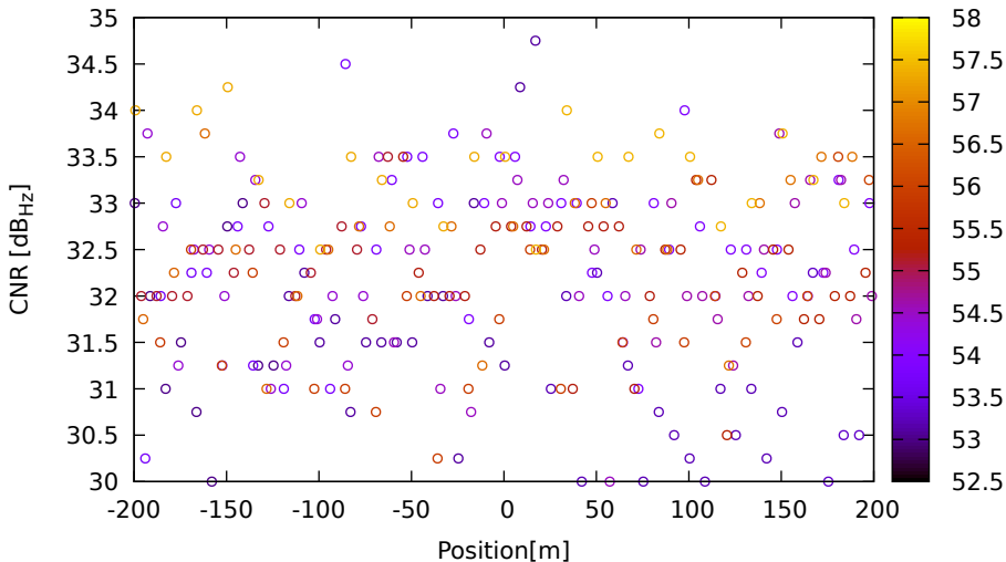
CNR vs position for E34 (E5a) on Xiaomi11T - DOY 262 jam. 2
