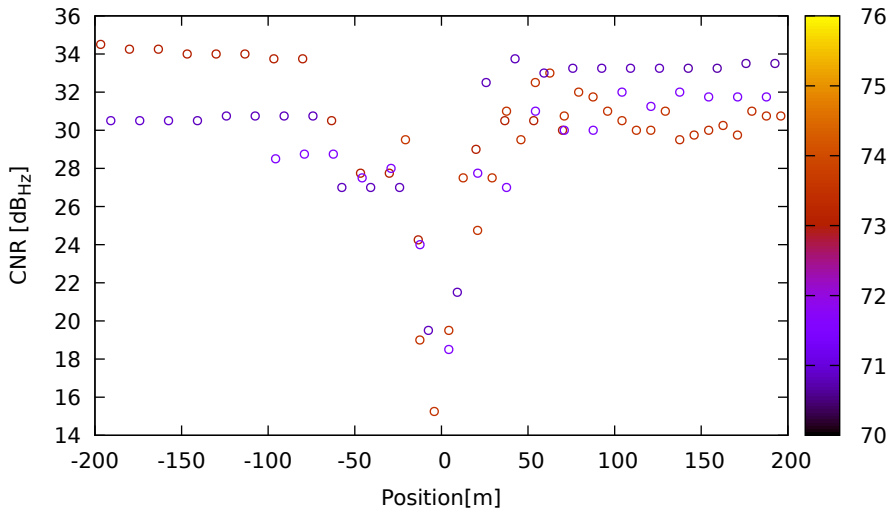
CNR vs position for E36 (E1) on Xiaomi11T - DOY 262 jam. 1
