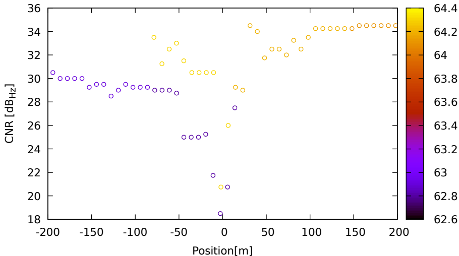
CNR vs position for E36 (E1) on Xiaomi11T - DOY 262 jam. 3
