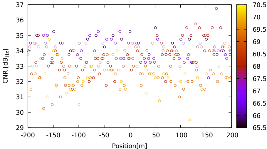
CNR vs position for E36 (E5a) on Xiaomi11T - DOY 262 jam. 2
