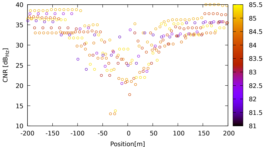
CNR vs position for G01 (L1) on Xiaomi11T - DOY 262 jam. 2
