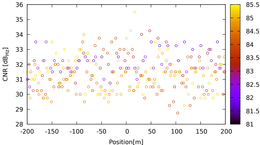
CNR vs position for G01 (L5) on Xiaomi11T - DOY 262 jam. 2
