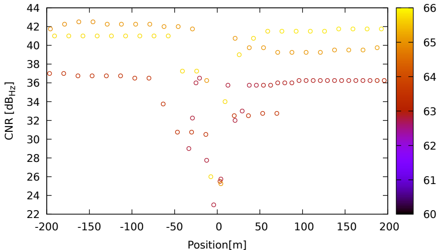
CNR vs position for G03 (L1) on Xiaomi11T - DOY 262 jam. 1
