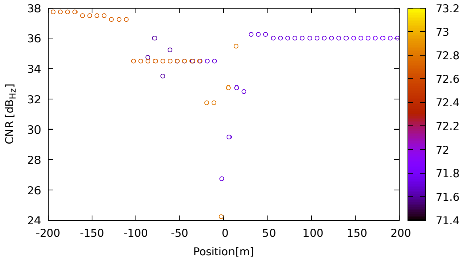
CNR vs position for G03 (L1) on Xiaomi11T - DOY 262 jam. 3
