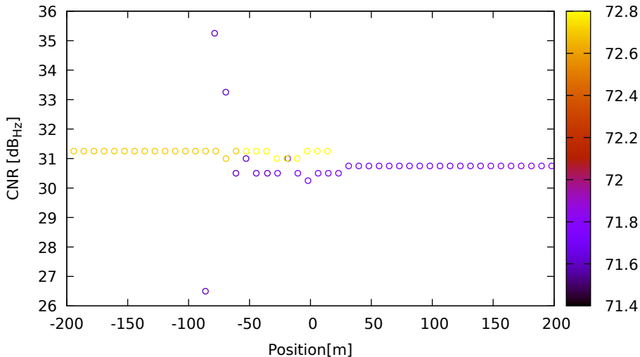
CNR vs position for G03 (L5) on Xiaomi11T - DOY 262 jam. 3
