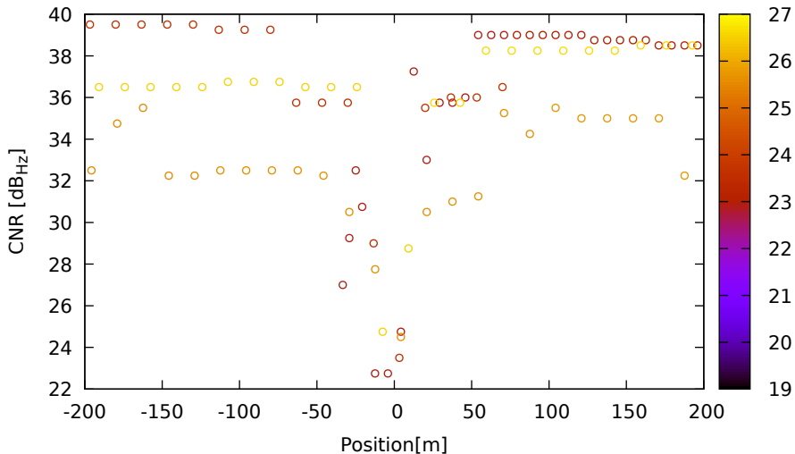
CNR vs position for G04 (L1) on Xiaomi11T - DOY 262 jam. 1
