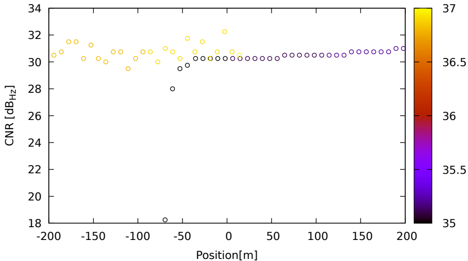
CNR vs position for G04 (L5) on Xiaomi11T - DOY 262 jam. 3
