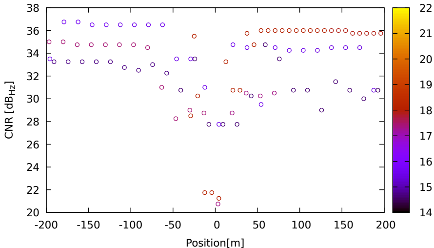
CNR vs position for G08 (L1) on Xiaomi11T - DOY 262 jam. 1
