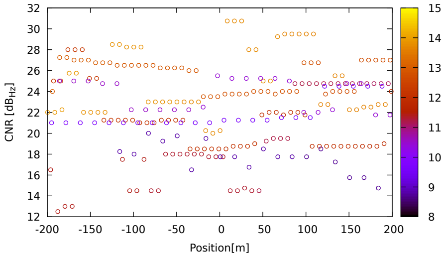
CNR vs position for G08 (L5) on Xiaomi11T - DOY 262 jam. 2
