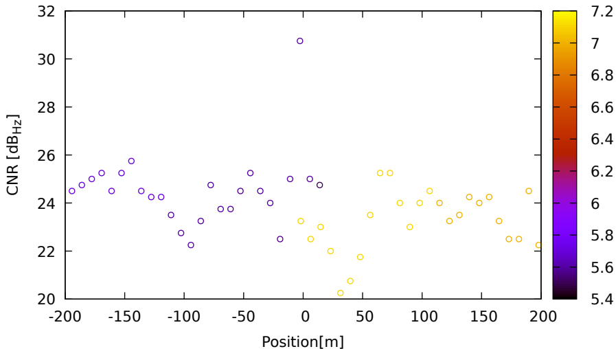
CNR vs position for G08 (L5) on Xiaomi11T - DOY 262 jam. 3
