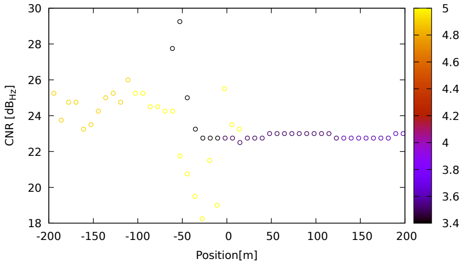
CNR vs position for G09 (L5) on Xiaomi11T - DOY 262 jam. 3
