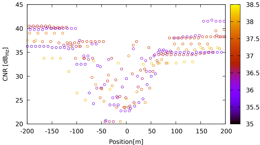
CNR vs position for G17 (L1) on Xiaomi11T - DOY 262 jam. 2
