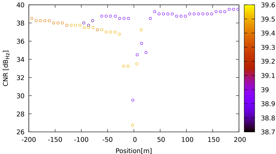
CNR vs position for G17 (L1) on Xiaomi11T - DOY 262 jam. 3
