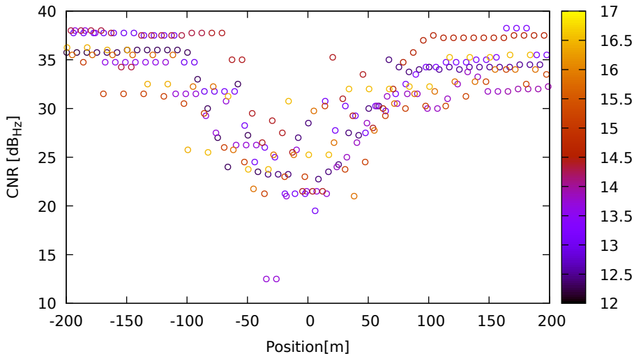
CNR vs position for G19 (L1) on Xiaomi11T - DOY 262 jam. 2
