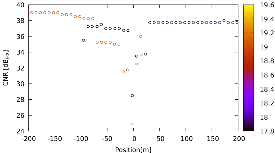
CNR vs position for G19 (L1) on Xiaomi11T - DOY 262 jam. 3
