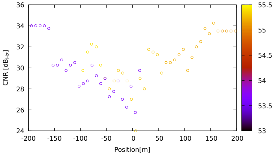
CNR vs position for G21 (L1) on Xiaomi11T - DOY 262 jam. 3
