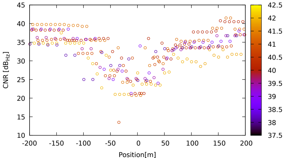
CNR vs position for G22 (L1) on Xiaomi11T - DOY 262 jam. 2
