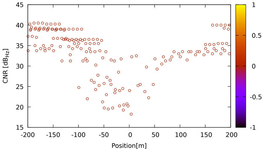
CNR vs position for G28 (L1) on Xiaomi11T - DOY 262 jam. 2
