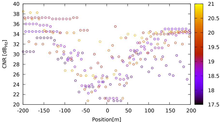
CNR vs position for G31 (L1) on Xiaomi11T - DOY 262 jam. 2
