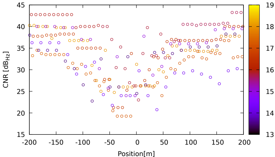
CNR vs position for G32 (L1) on Xiaomi11T - DOY 262 jam. 2
